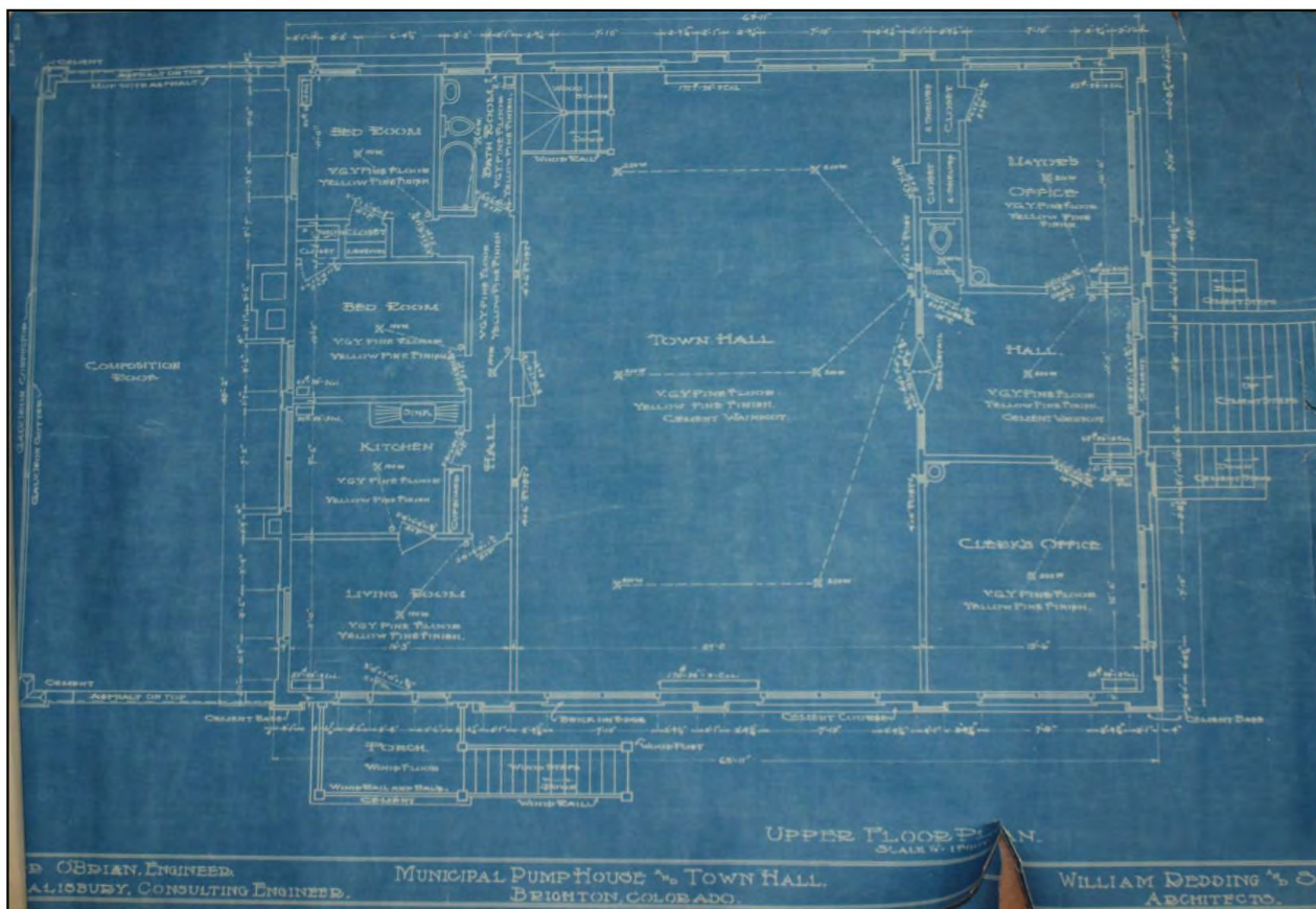
Figure 5. "Upper Floor Plan," 1918 blueprints, William Redding & Son, Architects. Source: City of Brighton, Historic Preservation Commission.
