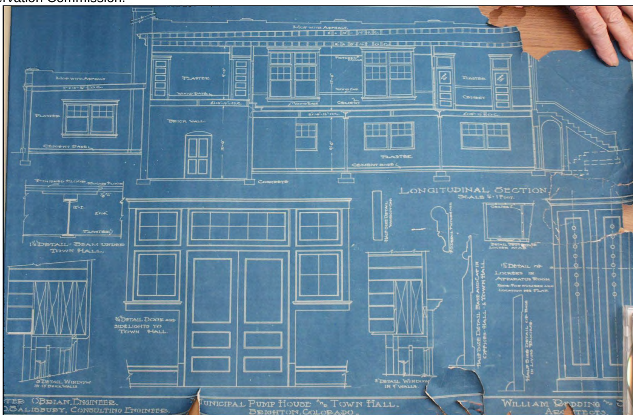
Figure 5. Elevation and details, 1918 blueprints, William Redding & Son, Architects. Source: City of Brighton, Historic Preservation Commission
